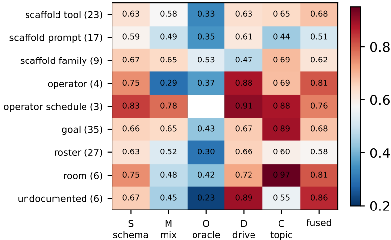
AUC: event window vs placebo window
