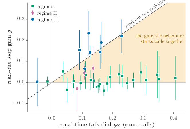
FIG. 21. The scheduler impostor, measured (H67). Each point is a goal period. The equal-time dial g_{eq} counts how much agents talk in the same calls. The read-out gain g counts only the response to a message that a call reads. In regime I (green squares) the equal-time dial is large, but the read-out gain is near zero. Agents talked together because the scaffold scheduled their calls together, not because they read each other. In regime III (blue circles) the two agree. Look at the orange gap between the green points and the diagonal: that gap is the impostor.
