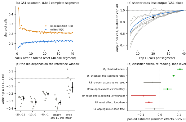
Second figure. Round 2. (a) G51 complete 40-call sawtooths: re-acquisition and write share by call after a forced reset, with the two-timescale fit. (b) Output per call under a cap of L calls, relative to 40, for nine periods (diamond: pooled Y(20)/Y(40) ). (c) The forced write dip against five reference windows (dots: periods; diamonds: pooled). (d) Pooled classifier check, recency-adjusted re-open excess and loop-lever effects.
