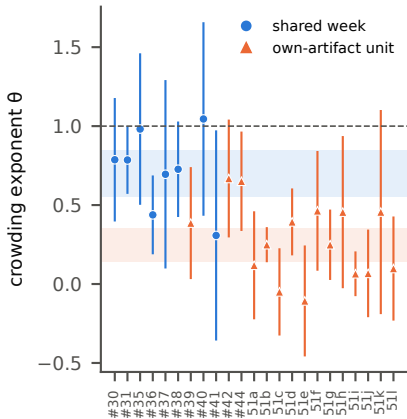
(a) project commits \propto n^\theta
