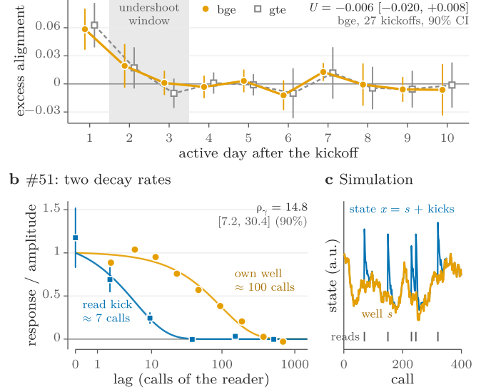
FIG. 6. A fast read kick on a slow, overdamped well (M16). (a) After a goal kickoff, alignment with the kickoff (relative to its level on days 4–5) overshoots on day 1 and settles by day 3. Nothing dips in the gray undershoot window ( U = -0.006 [-0.020, +0.008] , bge, 27 kickoffs, 90% CI; H125). Gray squares: the same with gte embeddings. (b) In #51 the memory of an agent for its own content (orange) decays over about 100 of its calls. The pull of a read (blue) decays in about 7 (H130). We divide each series by its fitted amplitude; thin lines are e^{-\gamma n} . (c) Simulation: state x = \text{slow well } s + \text{short kicks at reads (ticks)} . Look at the gap between the two curves in (b): one rate cannot describe both.
