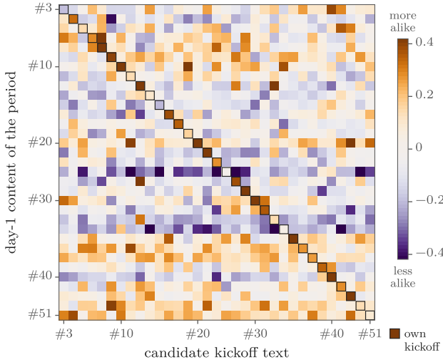
FIG. 5. The kickoff text is a field vector (M11, H54). Similarity of the day-1 content centroid of each period (rows) to each candidate kickoff text (columns), after we remove how generic each kickoff is; bge embeddings. Orange: more alike than average; purple: less. Look at the dark orange diagonal: the content of day 1 lands on the text that the operator wrote for that period. The own kickoff ranks first in 18/33 periods (Fig. 17).
