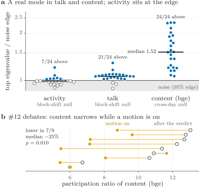
FIG. 7. Collective modes against a calibrated random-matrix edge (M17, H12). (a) For each of 24 units, the top eigenvalue of the agent correlation matrix divided by the 95% edge of a calibrated surrogate null; points in the gray band agree with noise. Activity mostly fails the trimmed block-shift null (7/24). Talk (21/24) and content (24/24, median ratio 1.52) carry a real mode. (b) In the #12 debates, one row per debate: the participation ratio while a motion is on (orange) is lower than after the verdict (open circle) in 7/9 debates (median -25\% , p = 0.010 ). Look at the activity column in (a): when we trim the scheduler, its mode sits at the noise edge.
