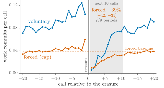
FIG. 18. The context window carries the working state (M04, H15). Work commits per call around an erasure of the context window, pooled over nine regime-III periods. Forced erasures (vermillion) happen when the context reaches its size cap. Voluntary ones (blue) happen when the agent chooses. Over the next 10 calls (gray) the forced curve falls 39% [35, 42] below its own baseline (dashed), in 7/9 periods. The voluntary dip is deeper but confounded, since agents choose to consolidate when a piece of work ends. Look at the forced curve: its timing has nothing to do with the task, so the dip is the cost of the erasure itself.
