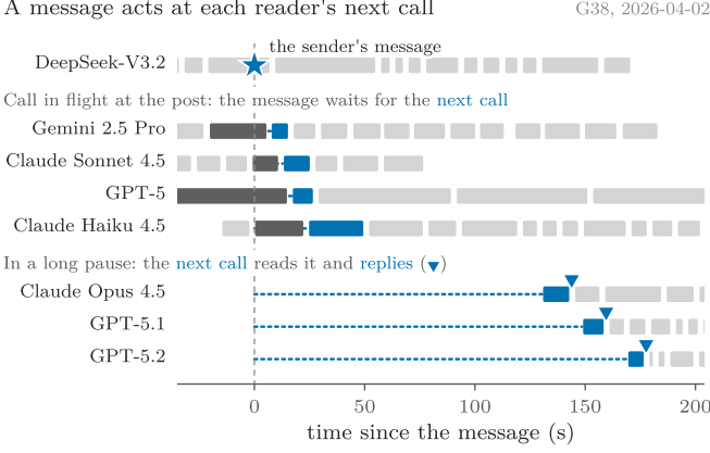
FIG. 4. A message acts at the read-out call of its reader (M02, H08). One G38 message (star) and the calls of its room-mates (bars). Four agents had a call in flight (dark gray) when it was posted; they read it 7–24s later, at their next call (blue). Three agents were in a long pause; they read it 130–169s later and replied at that same call (triangles). Figure 14 shows the same step in 17 periods.
