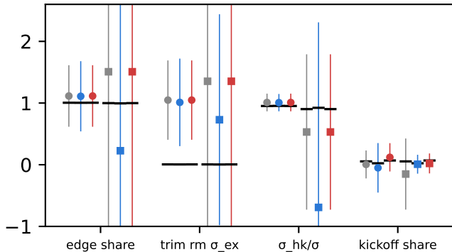
(a) synthetic: soft-label estimate \pm SD; bar = population
