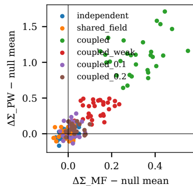
S3 collective excess per run
