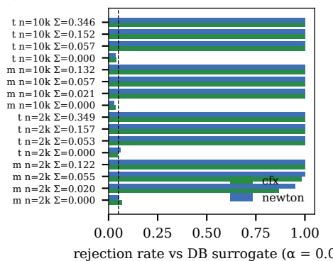
S3 collective excess per run
