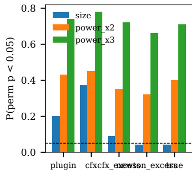
2c family test: equal true EP, families differ in n , stickiness S3 kinetic Potts N=15 , 5 d x 240
