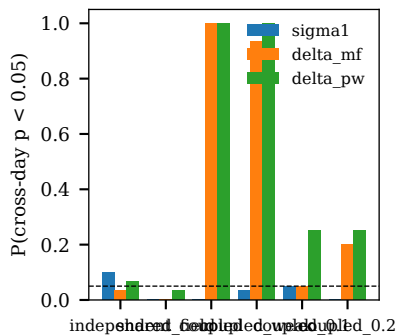
2c family test: equal true EP, families differ in n , stickiness S3 kinetic Potts N=15 , 5 d x 240
