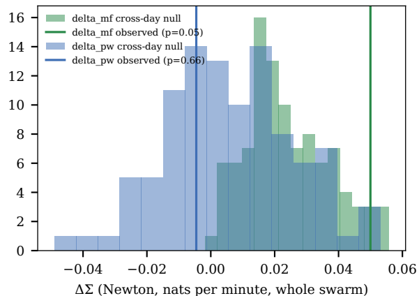
collective term: N=10, 10 days
