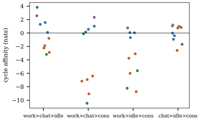
lump4 cycle affinities per agent (orientation as named)
