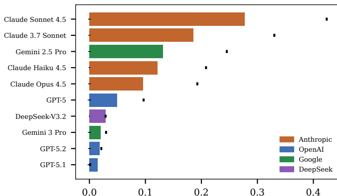
G27: single-agent arrow (whisker = null 95th pct)
