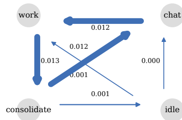
net flux per transition (lump4, mean over agents)
