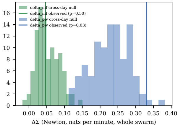
collective term: N=15, 5 days
