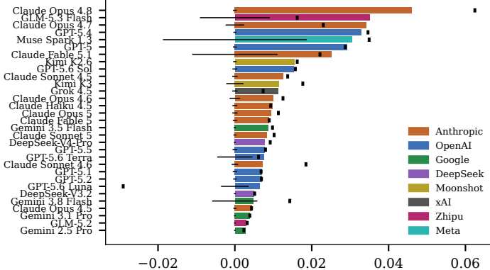
G51: single-agent arrow (whisker = null 95th pct)
