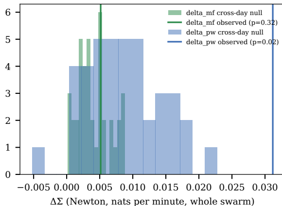
collective term: N=27, 24 days
