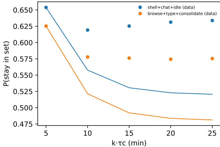
CK test ( m = 2 ); \max |\Delta| = 0.108
