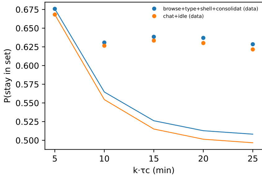
CK test ( m = 2 ); \max |\Delta| = 0.129
