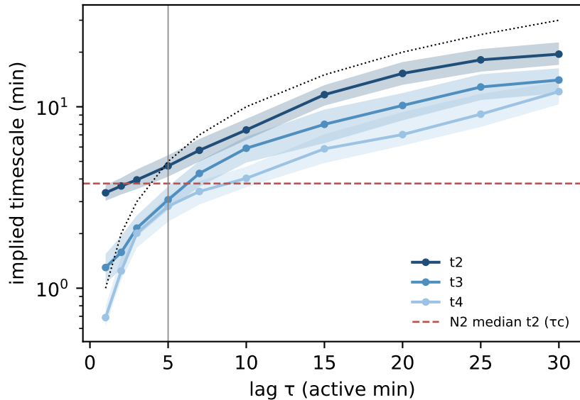
G19: ITS (non-reversible MLE)
