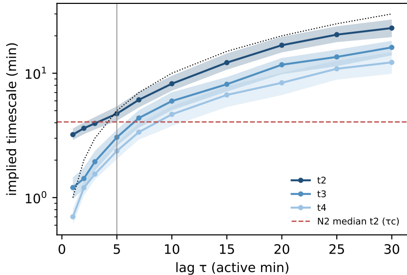
G20: ITS (non-reversible MLE)
