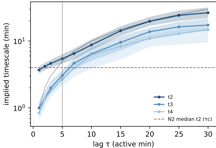
G21: ITS (non-reversible MLE)
