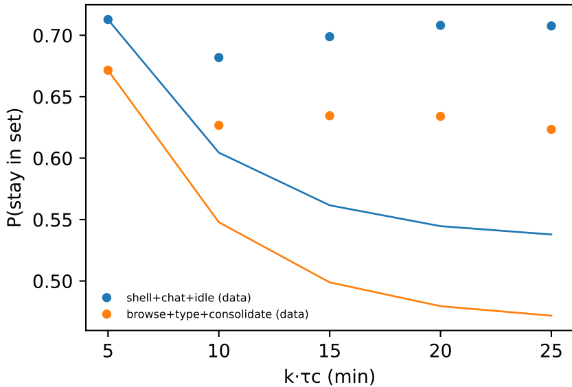
CK test ( m = 2 ); \max |\Delta| = 0.163
