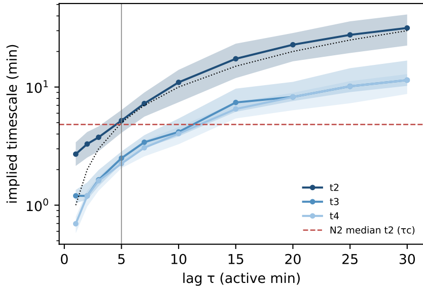
G23: ITS (non-reversible MLE)
