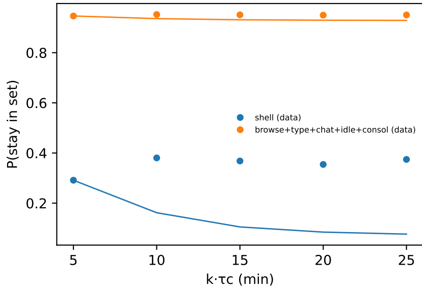
CK test ( m = 2 ); \max |\Delta| = 0.270
