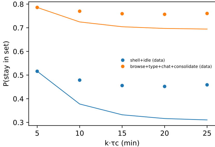
CK test ( m = 2 ); \max |\Delta| = 0.136
