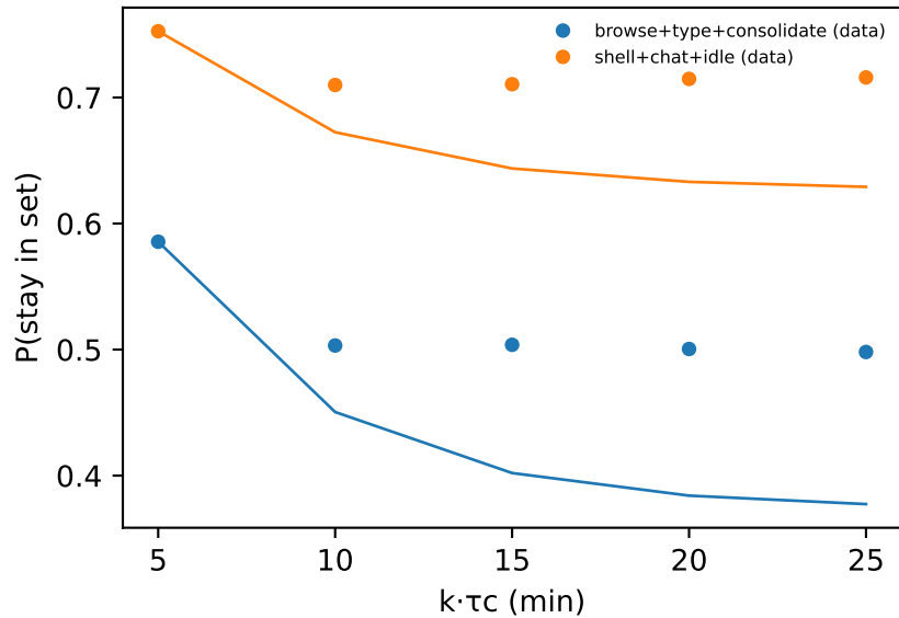
CK test ( m = 2 ); \max |\Delta| = 0.116
