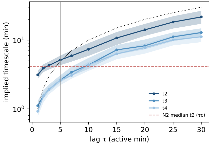
G26: ITS (non-reversible MLE)
