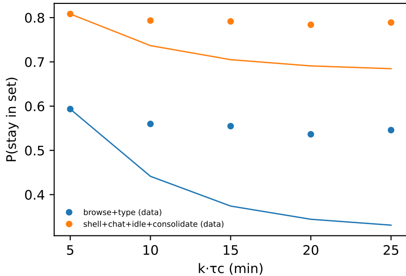
CK test ( m = 2 ); \max |\Delta| = 0.192
