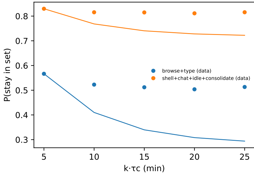
CK test ( m = 2 ); \max |\Delta| = 0.196
