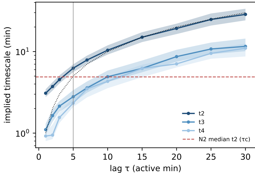
G31: ITS (non-reversible MLE)
