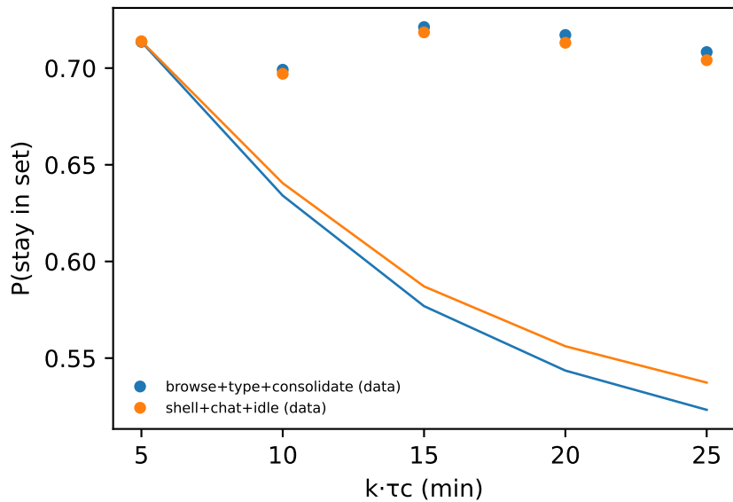
CK test ( m = 2 ); \max |\Delta| = 0.174
