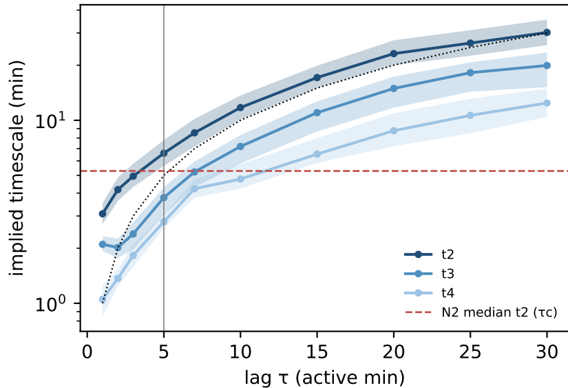
G39: ITS (non-reversible MLE)
