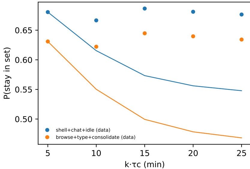
CK test ( m = 2 ); \max |\Delta| = 0.161
