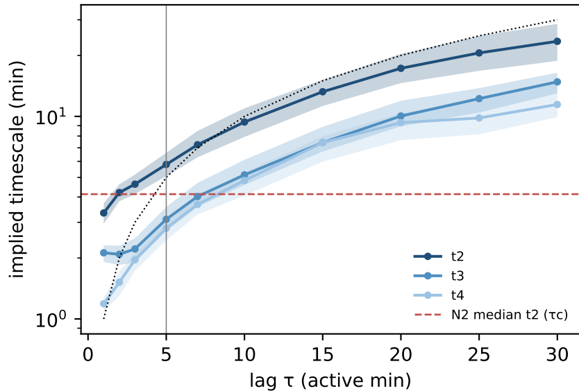
G42: ITS (non-reversible MLE)
