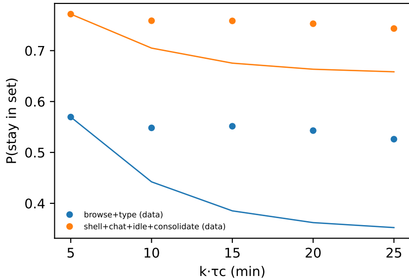
CK test ( m = 2 ); \max |\Delta| = 0.181
