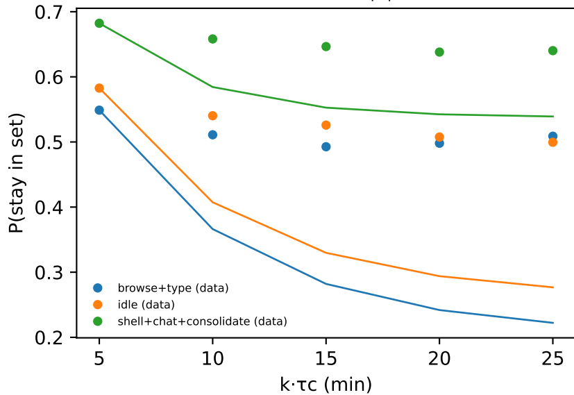
CK test ( m = 3 ); \max |\Delta| = 0.256
