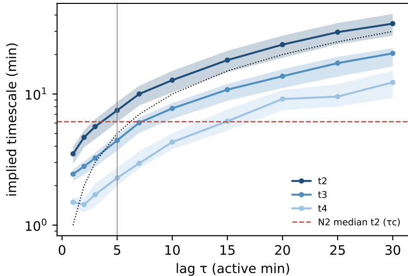
G44: ITS (non-reversible MLE)
