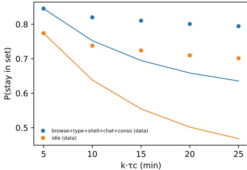
CK test ( m = 2 ); \max |\Delta| = 0.208
