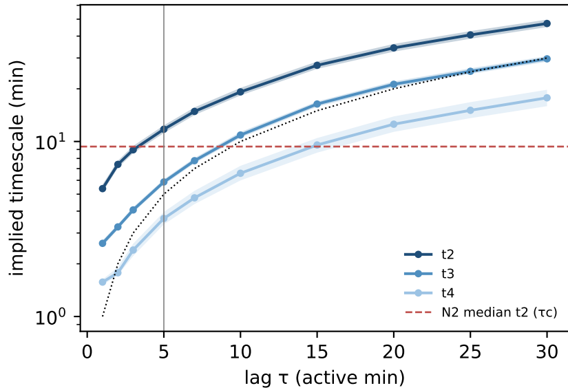
G51: ITS (non-reversible MLE)
