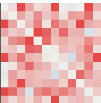
51d: content couplings J^c (N=12)
