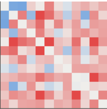
51a: content couplings J^c (N=12)
