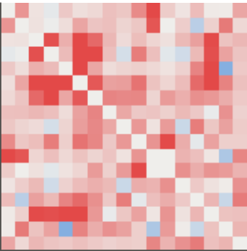
51b: content couplings J^c (N=17)
