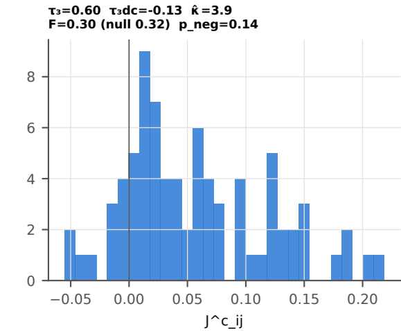
51c: content couplings J^c (N=13)
