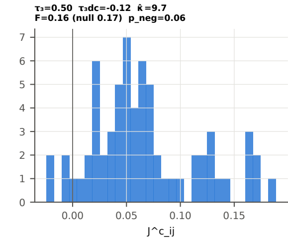
51d: content couplings J^c (N=12)
