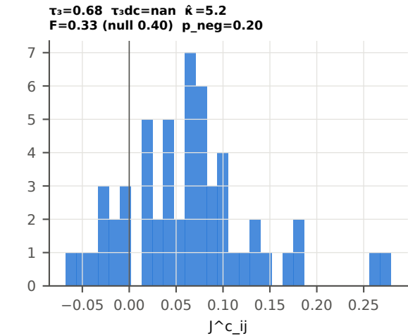
51e: content couplings J^c (N=11)
