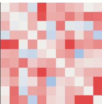
51e: content couplings J^c (N=11)
