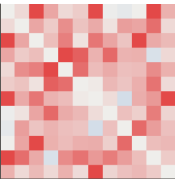
51d: content couplings J^c (N=12)
