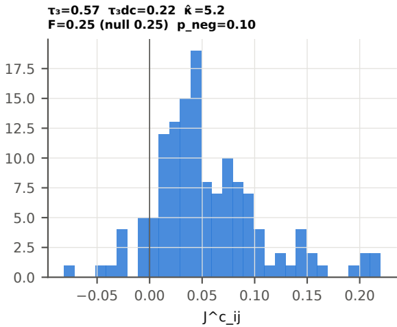
51b: content couplings J^c (N=17)
