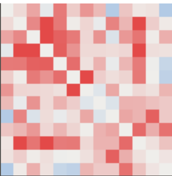
51c: content couplings J^c (N=13)
