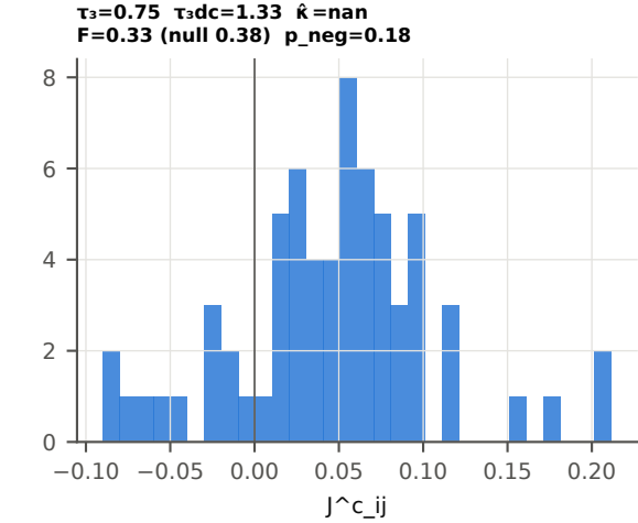
51a: content couplings J^c (N=12)
