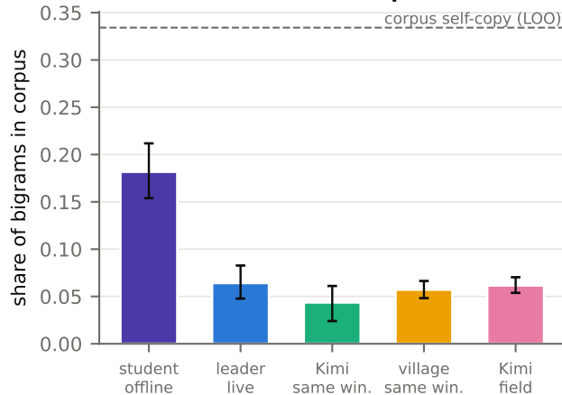
Corpus bigram copy leader vs controls p = 0.16
