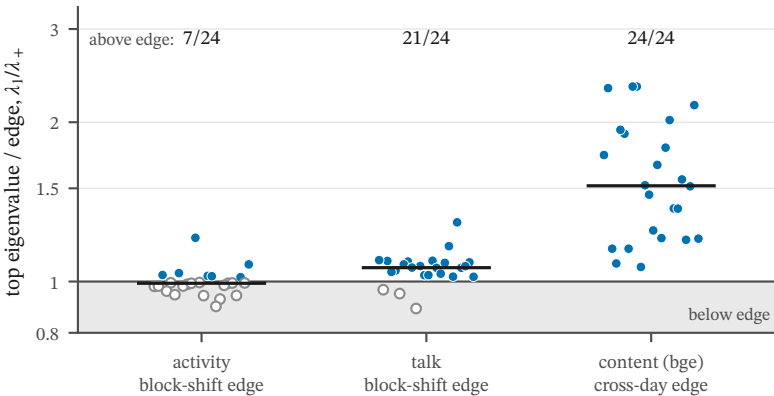
(a) collective mode per unit (24 units)
