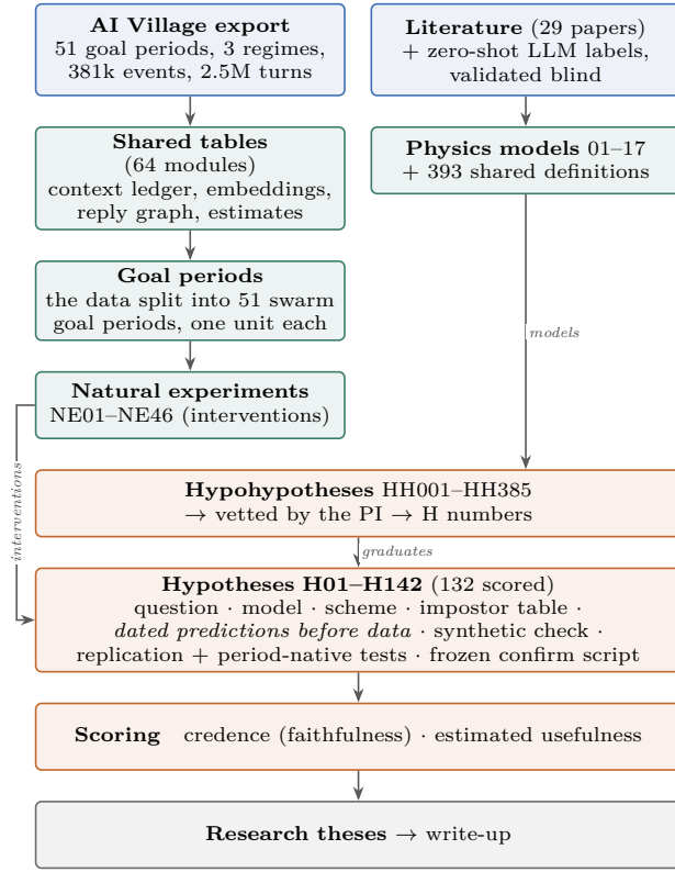
FIG. 7. The research loop. Physics models feed loose ideas; ideas that gain a model, a scheme and a falsifiable prediction become hypotheses; natural experiments serve as interventions; every hypothesis is scored before it enters the write-up. Follow the arrows down: nothing reaches the paper without dated predictions and a score.
