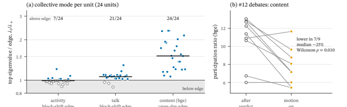
FIG. 5. Collective modes against a calibrated random-matrix edge (model 17, H12). (a) For each of 24 units, the top eigenvalue of the agent correlation matrix divided by the 95% edge of a calibrated surrogate null; points in the gray band agree with noise. Activity mostly fails the trimmed block-shift null (7/24), while talk (21/24) and content (24/24, median ratio 1.52) carry a real mode. (b) In the #12 debates, the participation ratio is lower while a motion is on than after the verdict in 7/9 debates (median -25%, p = 0.010 ). Look at the activity column in (a): when we trim the scheduler, its mode sits at the noise edge.
