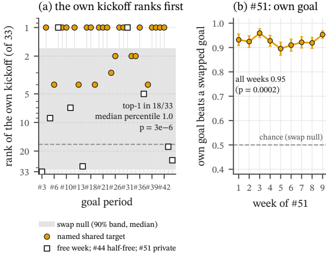
FIG. 15. The own kickoff is the target (model 11, H54). (a) Rank of the period’s own kickoff text among 33 candidates, by the similarity of Fig. 3: first in 18/33 periods, against a swap null whose median rank is 17 (gray band: 90%). Free weeks and private-goal periods (open squares) have no shared target and rank low, as they should. (b) In #51, where each agent had a private goal, an agent’s content matches its own goal text better than a swapped agent’s goal in 95% of pairs, every week (chance 0.5).
