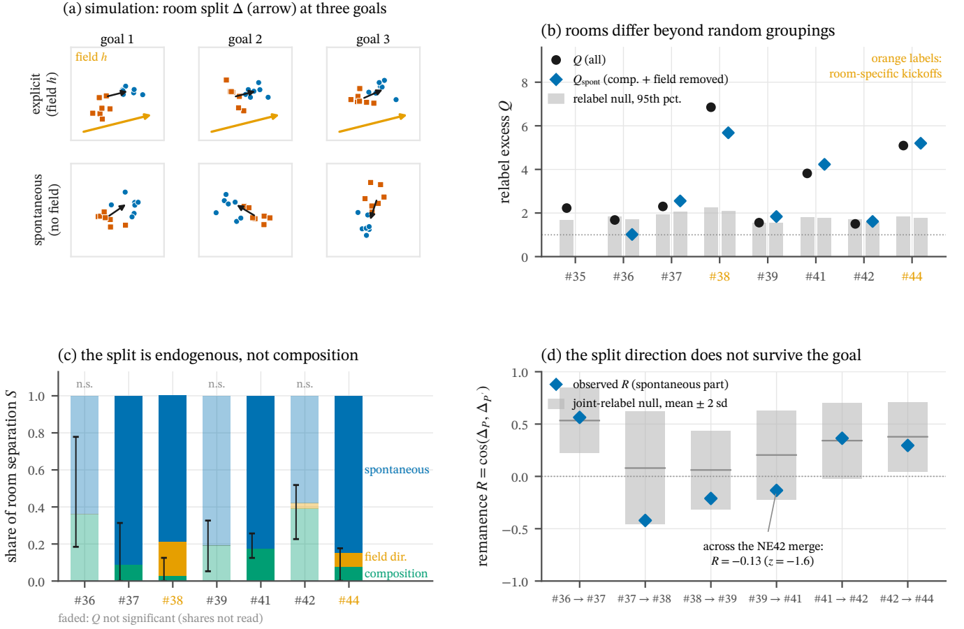
FIG. 20. The room content split is spontaneous and forms again at each goal (H100). (a) Two-block soft-spin simulation with and without a room field. (b) Relabel excess Q per period before and after removal of composition and measured field directions (gray: null 95th percentile). (c) Composition and spontaneous shares. (d) Persistence of the split direction between consecutive periods against the joint-relabel null. Look at (b) and (d) together: the rooms differ beyond random groupings in 5 of 7 regime-III periods (bge), but no split direction survives a goal change.
