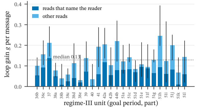
FIG. 13. The loop gain is small, and reads that name the reader carry about half of it (model 02, H67). Each bar is a regime-III unit (a goal period, or the part of one between two scaffold changes). The bar height is the read-out loop gain g : the number of extra talk calls that one message causes directly. The dark part comes from reads that name the reader; the light part from all other reads, which are far more numerous. Black lines: 95% CI. Look at the scale: every unit sits far below g = 1 , where echoes would run away.
