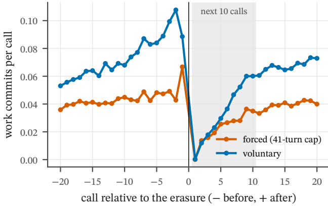
FIG. 16. The context window carries the working state (model 04, H15). Work commits per call around an erasure of the context window, pooled over nine regime-III periods: forced erasures (vermillion), which the scaffold triggers when the context reaches its size cap, and voluntary ones (blue), which the agent chooses. Over the next 10 calls (gray) the forced curve sits 39% [35, 42] below its own baseline. Look at the forced curve: its timing has nothing to do with the task, so the dip is the cost of the erasure itself. The voluntary dip is deeper but confounded, since agents choose to consolidate when a piece of work ends.
