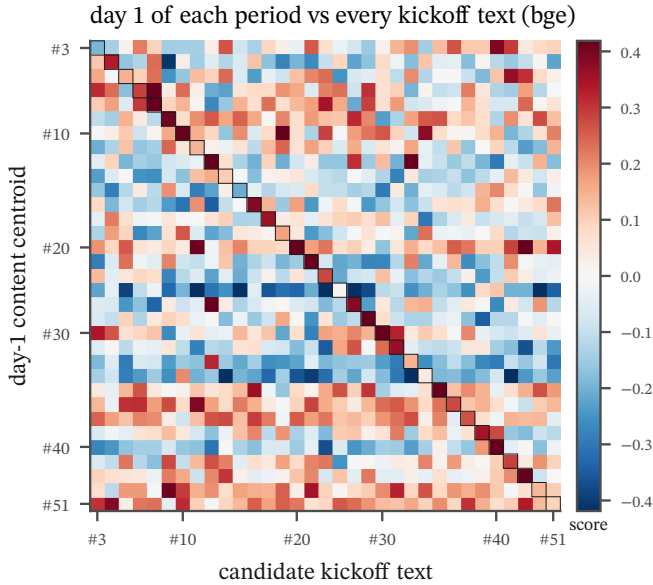
FIG. 3. The kickoff text is a field vector (model 11, H54). Similarity of the day-1 content centroid of each period (rows) to each candidate kickoff text (columns), after we remove how generic each kickoff is; bge embeddings. Look at the dark diagonal: the content of day 1 lands on the text that the operator wrote for that period. The own kickoff ranks first in 18/33 periods (Fig. 15).
