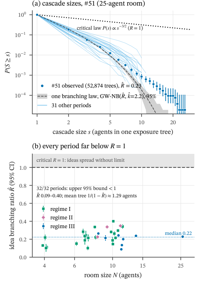
FIG. 18. Idea cascades are subcritical in every goal period (model 03, H34; round-1b data). (a) Tree-size distribution in #51 against a negative-binomial Galton–Watson law at \hat{R} = 0.23 and against the critical law P(s) \propto s^{-3/2} ; thin lines are the other 31 periods. (b) \hat{R} with 95% CI for the 32 non-reserved periods against room size. Look at panel (b): every upper bound sits below 1. Round 2 adds that the heavy tail is a spread of R across ideas.
