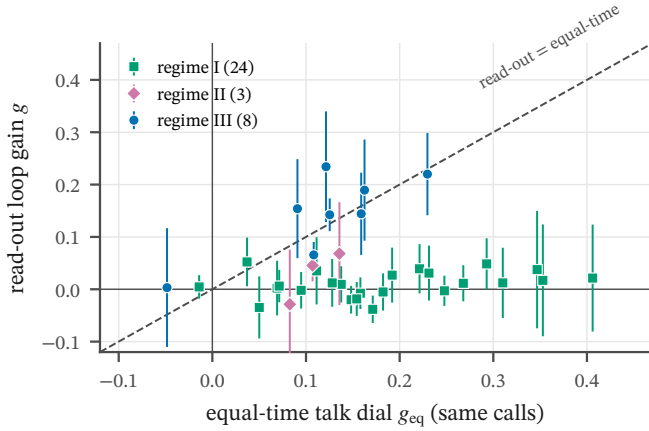
FIG. 19. The scheduler impostor, measured (H67). Each point is a goal period. The equal-time dial g_{eq} counts how much agents talk in the same calls; the read-out gain g counts only the response to a message that a call reads. In regime I (green squares) the equal-time dial is large while the read-out gain is near zero: agents talked together because the scaffold scheduled their calls together, not because they read each other. In regime III (blue circles) the two agree. Look at the gap between the green points and the diagonal: that gap is the impostor.
