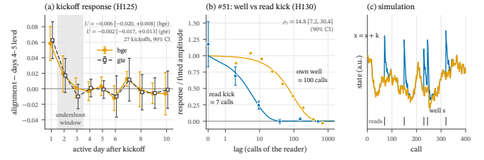
FIG. 4. A fast read kick on a slow, overdamped well (model 16). (a) After a goal kickoff, alignment with the kickoff (relative to its level on days 4–5) overshoots on day 1 and settles by day 3; nothing dips in the gray undershoot window ( U = -0.006 [-0.020, +0.008] , bge, 27 kickoffs, 90% CI; H125). (b) In #51 the memory of an agent for its own content (orange) decays over about 100 of its calls, while the pull of a read (blue) decays in about 7 (H130). We divide each series by its fitted amplitude; thin lines are e^{-\gamma n} . (c) Simulation: state x = \text{slow well } s + \text{short kicks at reads (ticks)} . Look at the gap between the two curves in (b): one rate cannot describe both.
