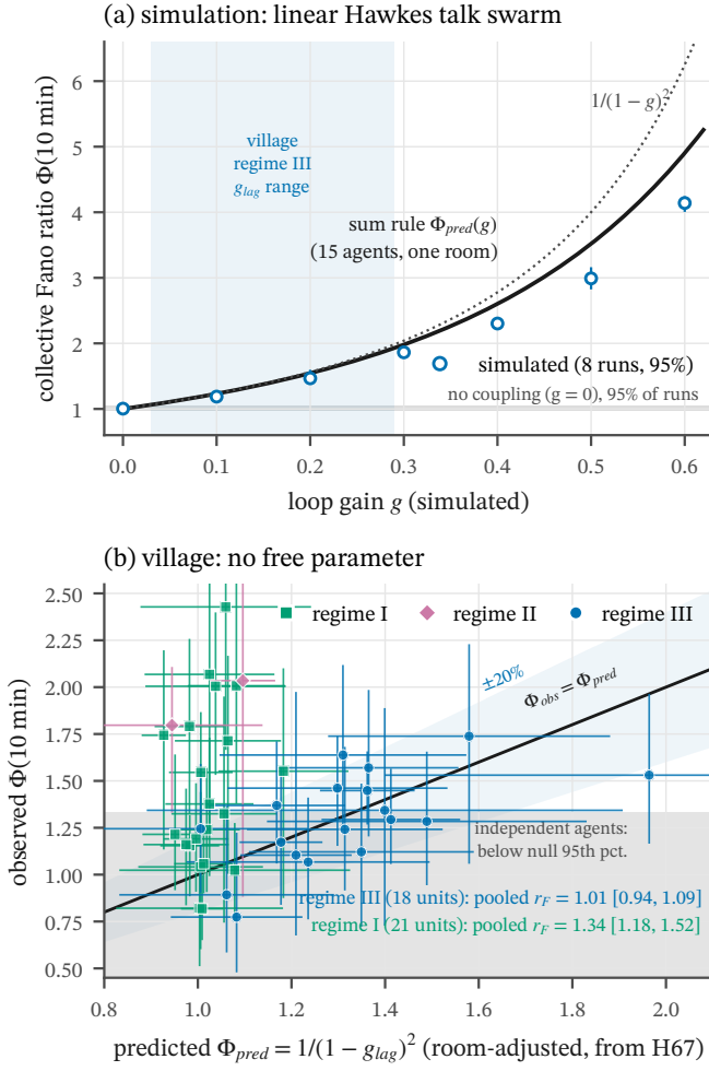
FIG. 14. A sum rule that links fluctuations to response for talk (models 02 and 09, H111; Eq. (2)). (a) In a simulated linear Hawkes swarm, the collective Fano ratio \Phi of 10-min talk counts follows 1/(1-g)^2 with no free parameter. (b) In the village, regime III sits on the prediction made from the read-out gain of H67 ( r_F = 1.01 [0.94, 1.09], 18 units). Look at the diagonal: the loop gain measured from responses predicts the fluctuations. Regime I lies above it ( r_F = 1.34 [1.18, 1.52]), for a reason we cannot explain.
