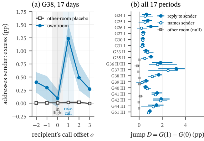
FIG. 12. The response starts at the read-out call (model 02, H08). (a) In G38, the excess chance that a call names the sender of a message, by the reader's call offset o from the read-out call ( o = 1 ). It is flat at the call in flight ( o = 0 , posted but not yet in the context) and jumps at o = 1 ; the other-room placebo (gray) stays at zero. (b) The jump D = G(1) - G(0) in 17 periods outside the reserved data, for replies (filled) and mentions (open), with the other-room null (gray squares). Look at the step between o = 0 and o = 1 in (a), and at the gray squares at zero in (b).
