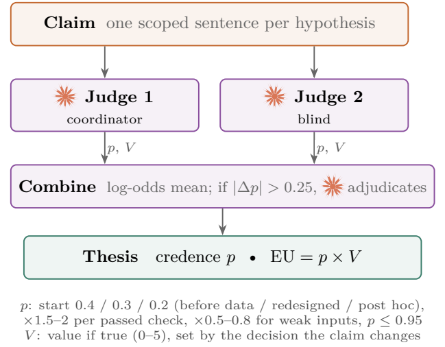
FIG. 8. Scoring. Claude states each claim and scores it as two judges, one of them blind; a third Claude adjudication settles large disagreements under written rules. The output is a credence p and an estimated usefulness EU = pV .
