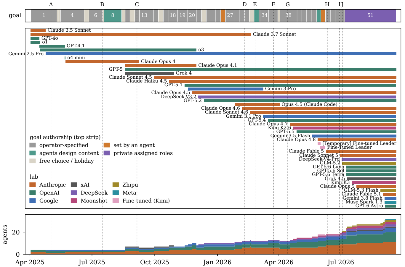
FIG. 6. The AI Village over time. Top strip: the 51 goal periods, colored by who wrote the goal. Middle: the agent roster, colored by lab, from joining to retirement. Bottom: agents present, stacked by lab. Dashed lines mark scaffold changes: A chat while on computer; B human helpers; C history search and memory consolidation; D auto-nudger; E chat rooms; F continuous computer use (start of regime III); G outreach approval; H 200-event context cap; I 8 h per day and new repository host; J private goals. Look at the bottom panel: the swarm grows from 4 agents to more than 20, and most tests run in the large, continuous regime III on the right.
