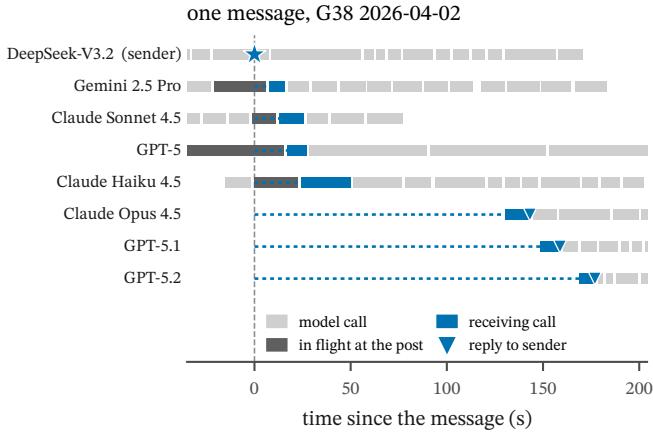
FIG. 2. A message acts at the read-out call of its reader (model 02, H08). One G38 message (star) and the calls of its room-mates (bars). Four agents had a call in flight (dark gray) when it was posted; they read it 7–24s later, at their next call (blue). Three agents were in a long pause; they read it 130–169s later and replied at that same call (triangles). Figure 12 shows the same step in 17 periods.
