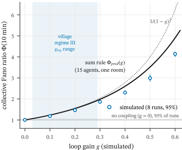
(a) simulation: linear Hawkes talk swarm
