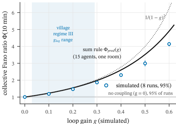
(a) simulation: linear Hawkes talk swarm
