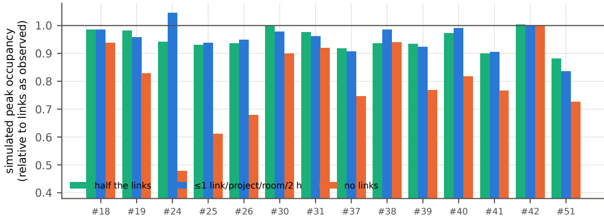
Counterfactual link throttling: peak number of agents on one project
