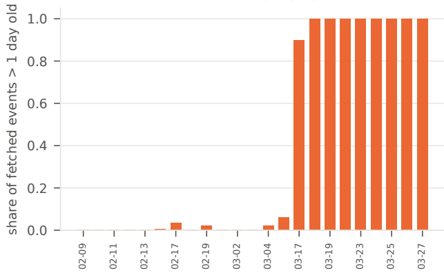
(a) Claude Code agent: history replay from 03-17
