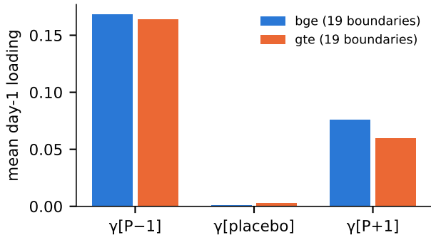
(a) past vs future vs placebo centroid
