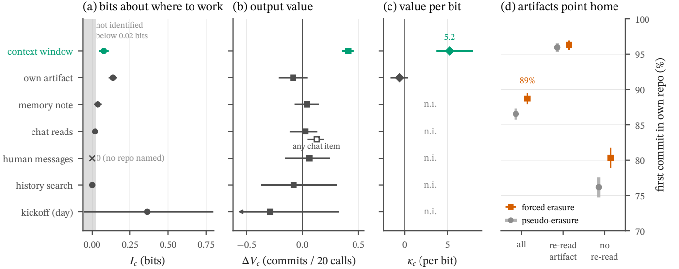
FIG. 13. The \kappa table: only the context window buys commits per bit (model 04, H87 with H70). Each row is a channel at its natural scramble (forced erasures; the kickoff for the last row), with agent-day paired bootstrap 95% intervals. (a) Bits about where to work. (b) Output value lost. (c) Value per bit. (d) After an erasure agents return to their own repository. Look at panel (c): only the context window has an identified, positive value per bit ( \kappa_C = 5.2 [3.8, 7.9]); “n.i.” marks rows below the 0.02-bit identification floor.
