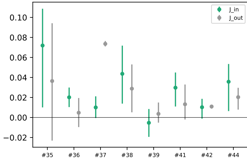
H05-MF block couplings, active spins (day-bootstrap 95% CI)
