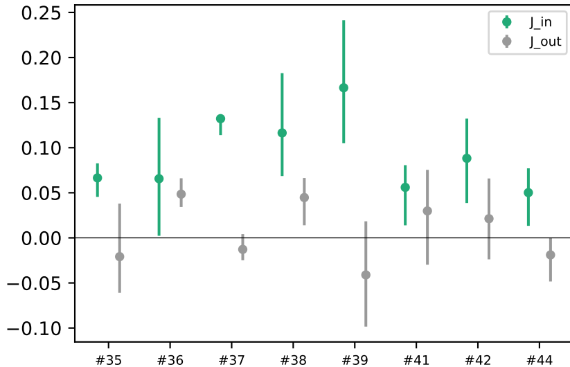
H05-MF block couplings, talk spins (day-bootstrap 95% CI)
