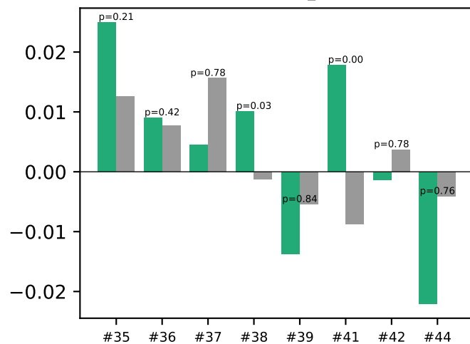
kinetic-Ising J_{\text{sym}}
