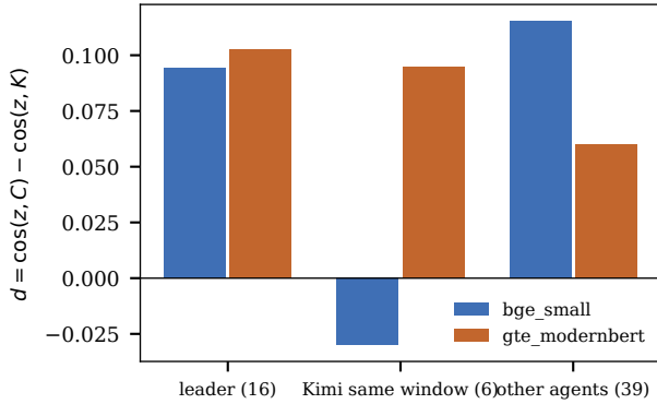
Second figure. Embedding-level proximity d = \cos(z, \bar{z}_{corpus}) - \cos(z, \bar{z}_{Kimi\ field}) in regime-III whitened space for the leader’s 16 live messages, the same-window Kimi K2.6 (6) and the other #best
