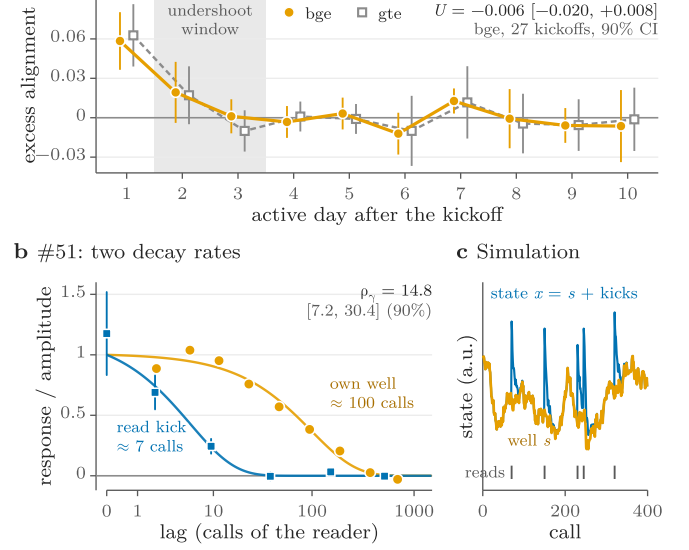
FIG. 5. A fast read kick on a slow, overdamped well (model 16). (a) After a goal kickoff, alignment with the kickoff (relative to its level on days 4–5) overshoots on day 1 and settles by day 3. Nothing dips in the gray undershoot window ( U = -0.006 [-0.020, +0.008] , bge, 27 kickoffs, 90% CI; H125). Gray squares: the same with gte embeddings. (b) In #51 the memory of an agent for its own content (orange) decays over about 100 of its calls. The pull of a read (blue) decays in about 7 (H130). We divide each series by its fitted amplitude; thin lines are e^{-\gamma n} . (c) Simulation: state x = \text{slow well } s + \text{short kicks at reads} (ticks). Look at the gap between the two curves in (b): one rate cannot describe both.
