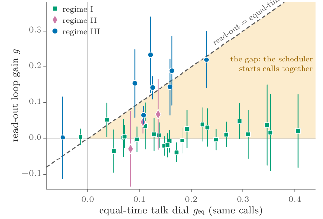
FIG. 20. The scheduler impostor, measured (H67). Each point is a goal period. The equal-time dial g_{eq} counts how much agents talk in the same calls. The read-out gain g counts only the response to a message that a call reads. In regime I (green squares) the equal-time dial is large, but the read-out gain is near zero. Agents talked together because the scaffold scheduled their calls together, not because they read each other. In regime III (blue circles) the two agree. Look at the orange gap between the green points and the diagonal: that gap is the impostor.
