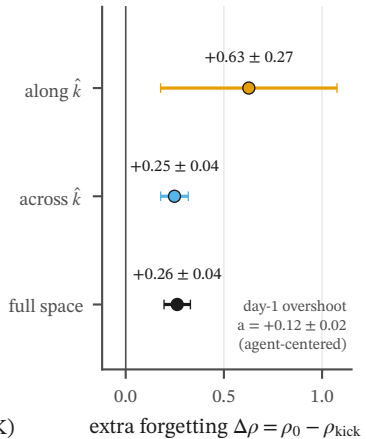
(c) the well is stiffer along \hat{k}
