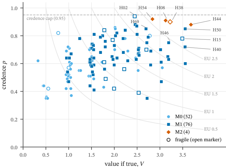
132 scored claims (median p = 0.64 )
