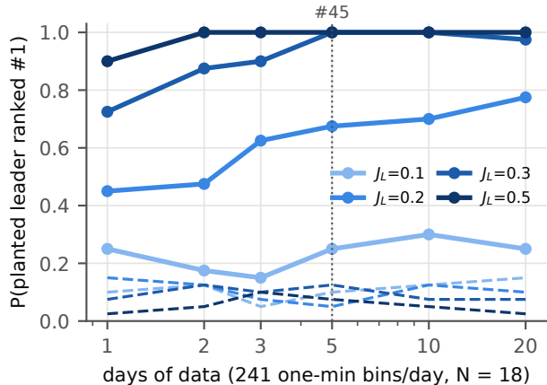
Leader ranked #1: KI-1 (solid) vs EQ-PL (dashed)
