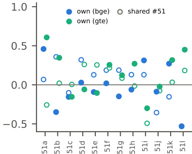
(b) #51: private fields, g_2 \approx 0
