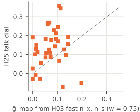
(c) unfitted mapping
