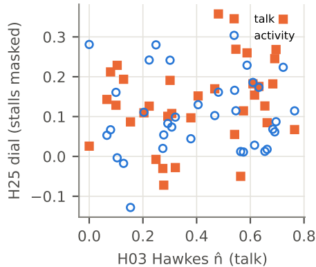
(b) vs Hawkes branching ratio
