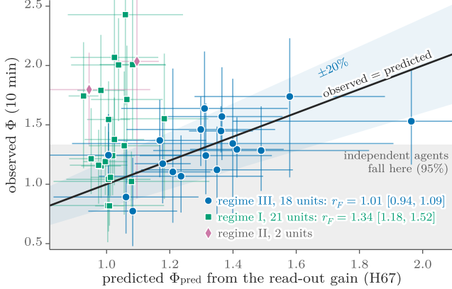
FIG. 16. A sum rule that links fluctuations to response for talk (models 02 and 09, H111; Eq. (2)). (a) In a simulated linear Hawkes swarm, the collective Fano ratio \Phi of 10-min talk counts follows 1/(1-g)^2 (room-adjusted for 15 agents) with no free parameter. (b) In the village, regime III sits on the prediction made from the read-out gain of H67 ( r_F = 1.01 [0.94, 1.09], 18 units). Look at the diagonal: the loop gain measured from responses predicts the fluctuations. Regime I lies above it ( r_F = 1.34 [1.18, 1.52]), for a reason we cannot explain.
