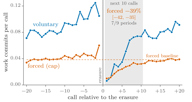
FIG. 18. The context window carries the working state (model 04, H15). Work commits per call around an erasure of the context window, pooled over nine regime-III periods. Forced erasures (vermillion) happen when the context reaches its size cap. Voluntary ones (blue) happen when the agent chooses. Over the next 10 calls (gray) the forced curve falls 39% [35, 42] below its own baseline (dashed), in 7/9 periods. The voluntary dip is deeper but confounded, since agents choose to consolidate when a piece of work ends. Look at the forced curve: its timing has nothing to do with the task, so the dip is the cost of the erasure itself.
