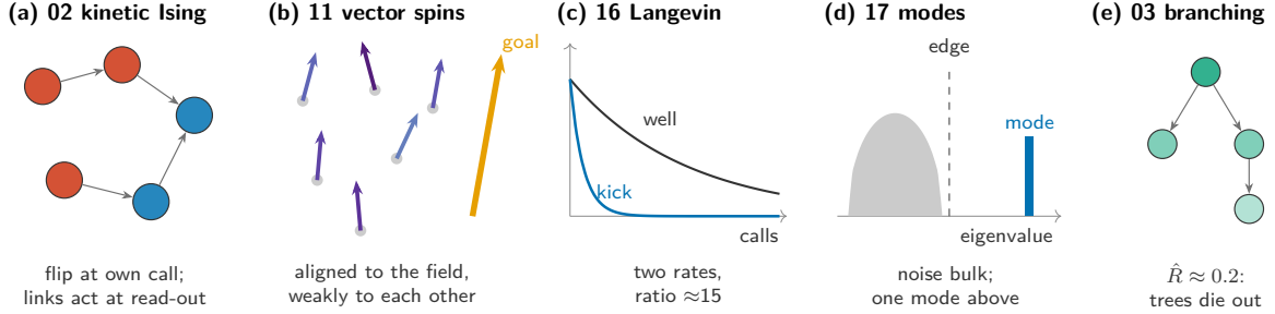
FIG. 13. The useful model families, from the most to the least useful. (a) Kinetic Ising with read-out coupling (model 02): each agent is a two-state spin (two colors) that updates only at its own calls; links act at the read-out call. (b) Vector spins (model 11): each agent’s content is an arrow (color = angle); the goal is a strong field (orange), so the arrows align with it and only weakly with each other. (c) Langevin relaxation (model 16): a read kick decays about 15 times faster than the agent’s own well. (d) Collective modes (model 17): a mode counts only above the calibrated noise edge. (e) Branching (model 03): idea trees die out, \hat{R} \approx 0.2 .
