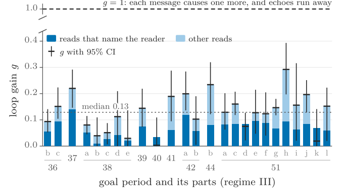
FIG. 15. The loop gain is small, and reads that name the reader carry about half of it (model 02, H67). Each bar is a regime-III unit (a goal period, or the part of one between two scaffold changes). The bar height is the read-out loop gain g : the number of extra talk calls that one message causes directly. The dark part comes from reads that name the reader, and the light part from all other reads, which are far more numerous. In three units the named part alone exceeds g , so there the other reads add nothing. Black lines: 95% CI (cut at 0). The dashed line at the top is g = 1 , where echoes would run away. Look at the scale: every unit sits far below g = 1 .
