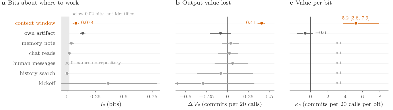
FIG. 19. The \kappa table: only the context window buys commits per bit (model 04, H87). Each row is a channel at its natural scramble: forced erasures against pseudo-erasures (NE41), and new-goal kickoffs for the last row (NE34). Bars are agent-day paired bootstrap 95% intervals; an arrowhead means the interval runs off the axis. (a) Bits about where the agent works next, beyond its identity. Rows whose lower bound is under 0.02 bits (gray strip) are not identified. Human messages name no repository, so they carry 0 bits. (b) Work commits per 20 calls lost when the channel is scrambled. (c) Value per bit, \kappa_c = \Delta V_c / I_c , for identified rows; “n.i.” marks the others. Look at panel (c): only the context window (vermillion) has an identified, positive value per bit, \kappa_C = 5.2 [3.8, 7.9]. The own artifact carries the most bits but no value ( \kappa_A = -0.6 ).
