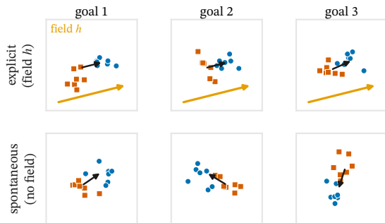
(a) simulation: room split \Delta (arrow) at three goals
