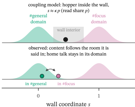
(a) schematic: domains and the wall
