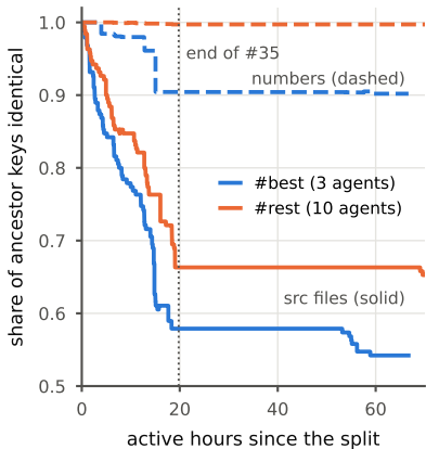
(a) Vertical: code drifts gradually, content jumps (in #best only)
