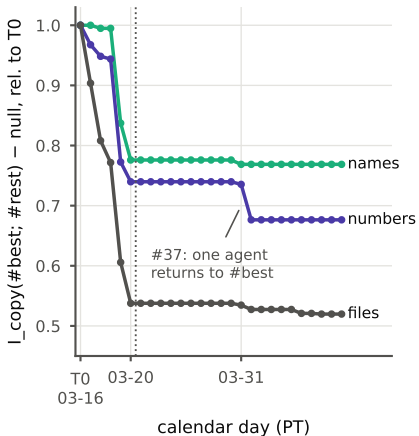
(b) Horizontal: decays through #35, then freezes (P4)
