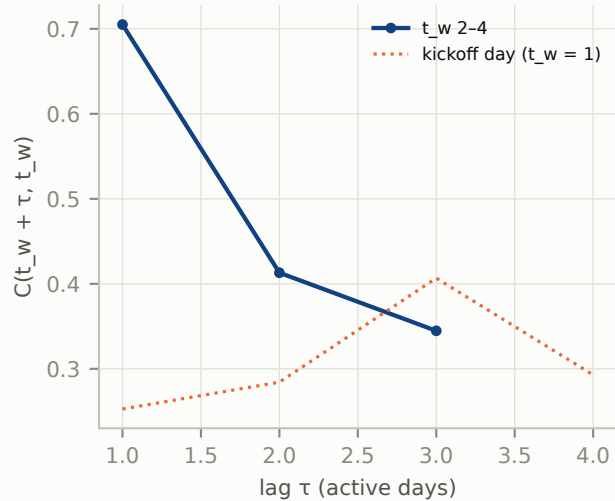
#5: C by age band
