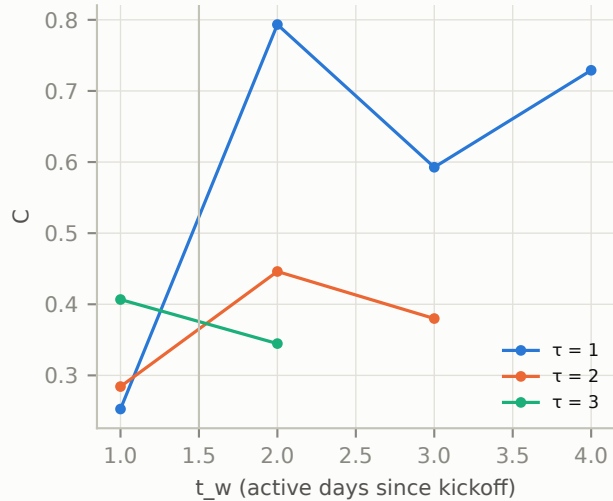
A = +0.357 (p = 0.287); A_late = +0.474
