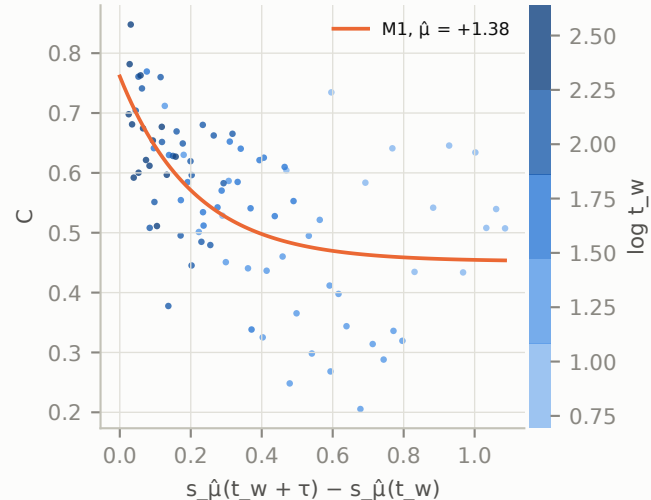
collapse, \hat{\mu} CI [-0.12, +2.43]
