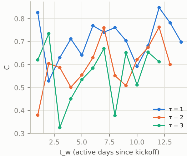
A = +0.071 ( p = 0.120 ); A_{\text{late}} = +0.040
