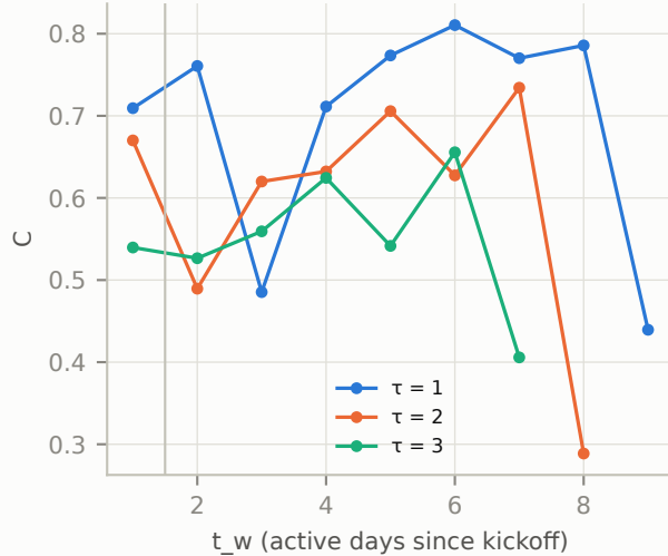
A = -0.002 ( p = 0.473 ); A_{\text{late}} = -0.825
