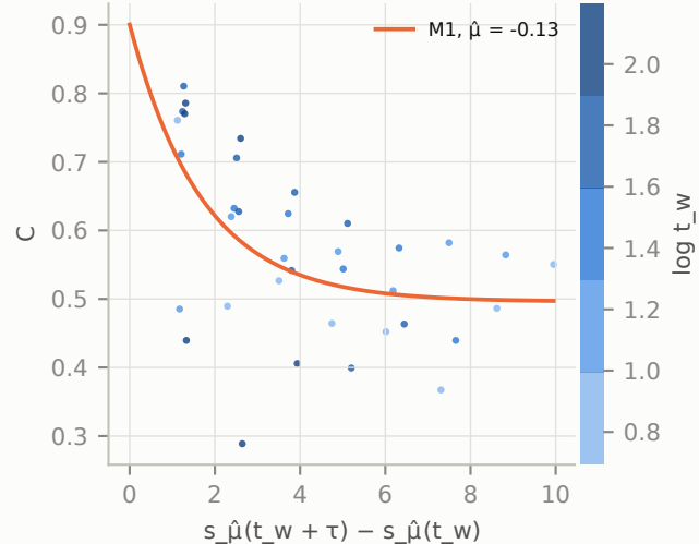
collapse, \hat{\mu} CI [-2.75, +1.59]
